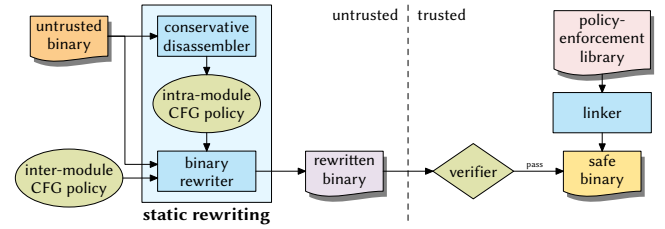
Figure 5: REINS system architecture
