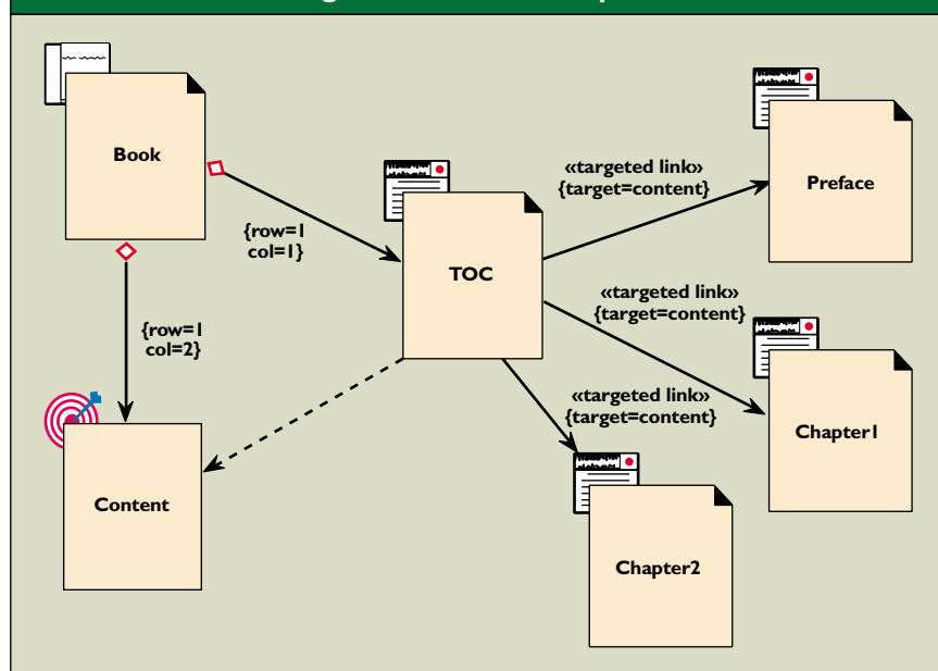
Figure 5. Frames example.
