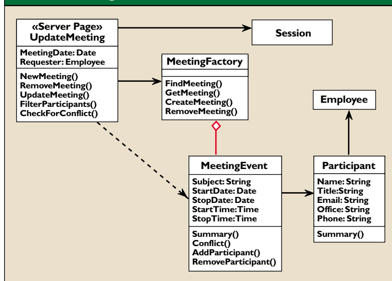
Figure 3. Server collaborations.
