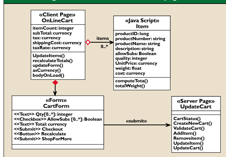
Figure 4. Forms submit to server pages.
