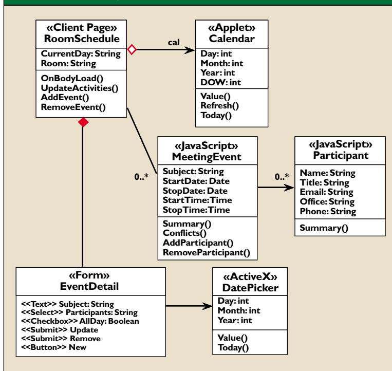
Figure 2. Client collaborations.
