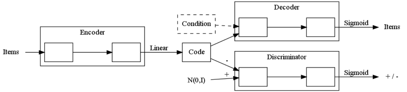
Figure 2: Adversarial autoencoder for item-based recommendations. Each edge resembles a parametrized mapping f(Wx + b) with activation function f and parameters W, b . When not labeled differently, the activation function is rectified linear followed by dropout.
