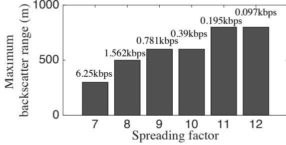
Figure 14: Maximum backscatter range on different bit rate settings. The outdoor temperature is 5° C.
