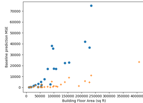
Figure 9: Comparing the mean squared error of building energy consumption prediction using the baseline from [21] trained and evaluated on summer months (+) versus winter months (•).
