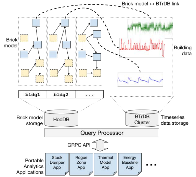
Figure 1: Mortar architecture
