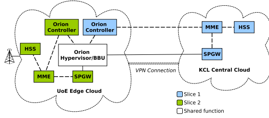
Figure 5: Neutral-host use case setup with 2 tenants
