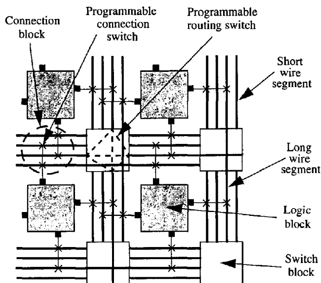
Figure 2: An island-style FPGA (from [2]).
