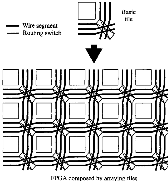
Figure 9: Tiled layout to implement FPGA of Figure 8.
