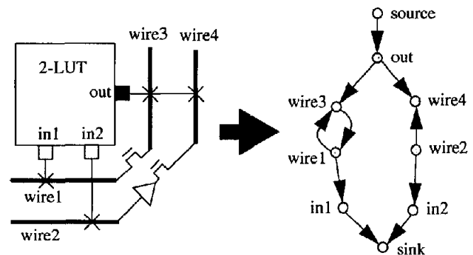
Figure 4: Modelling FPGA routing as a directed graph.
