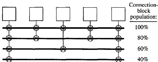
Figure 3: Possible connection-block population values for length 5 wire segments.
