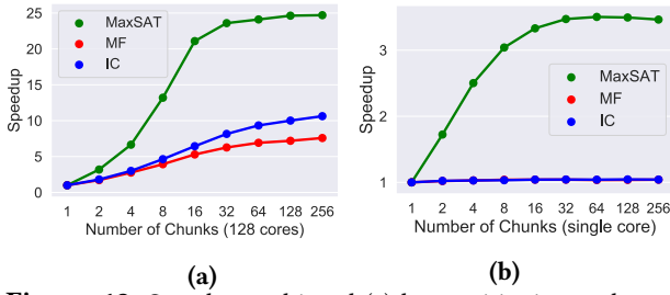
Figure 12: Speed up achieved (a) by partitioning and parallel processing on 128 cores; (b) by partitioning on a single core.
