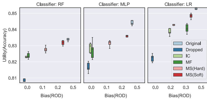
Figure 7: Performance of CAPUCHIN on Adult data.
