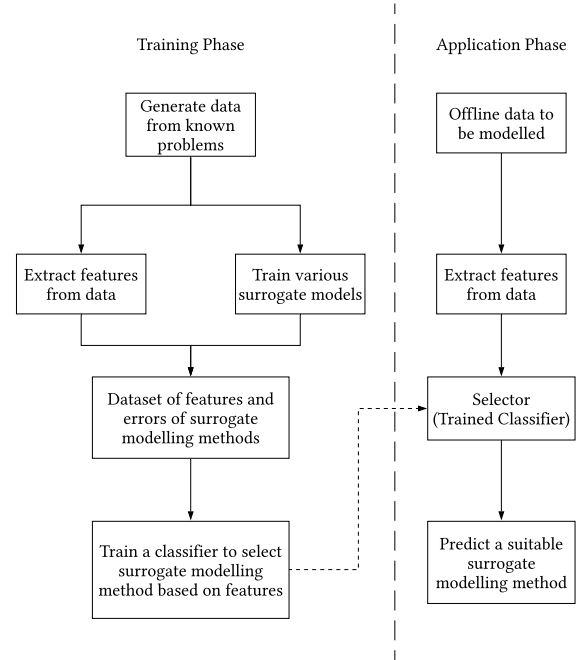
Figure 1: Automatic selection of surrogate modelling techniques based on optimization features.
