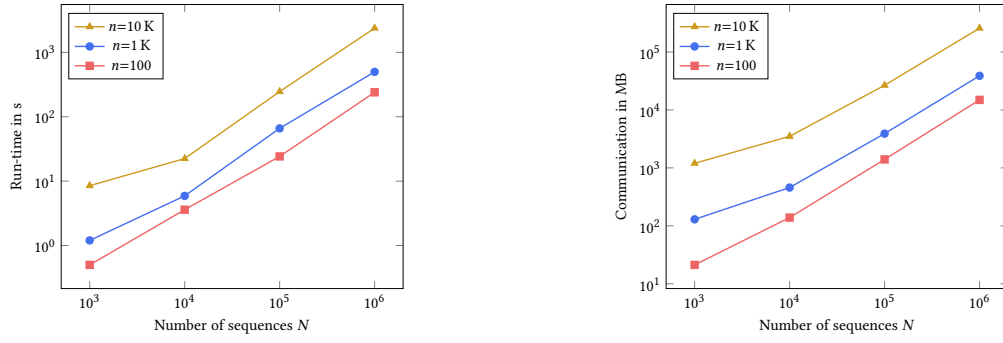
Figure 5: Large-scale benchmarks of our Similar Sequence Query algorithm for N sequences of length n , LUT width w=30 , number of data providers \psi=10 , number of most similar sequence queries k=10 , block size b=5 , and padded block size b'=16 . Numbers are given in Table 5.
