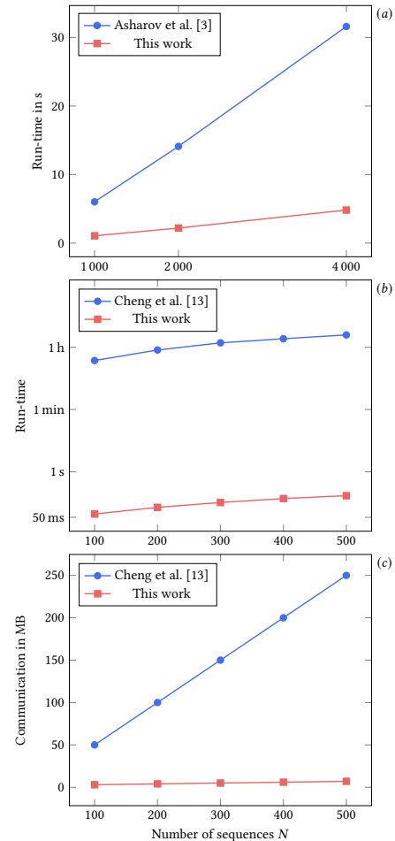
Figure 4: (a) A run-time comparison of our Similar Sequence Query algorithm with that of Asharov et al. [3] with sequence length n=3470 , number of nearest sequences k=5 , block length b=4 , padded block length b'=16 , and number of data providers \psi=1 performed locally for different numbers of sequences N and LUT widths \omega . (b,c) A run-time and communication comparison of our SSQ algorithm with that of Cheng et al. [13] with n=500 , b=5 , k=10 , \omega=20 , and number of blocks t=20 . Numbers are given in Tables 2 (a) and 4 (b,c).
