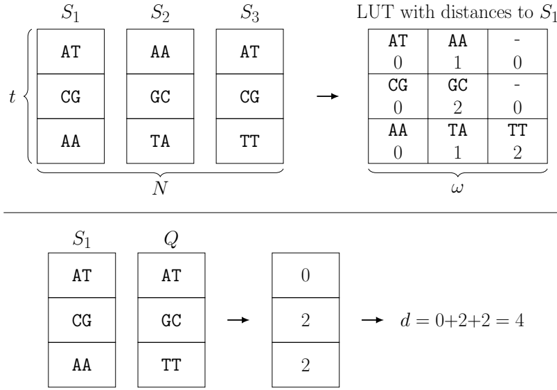
Figure 1: Example for computation of the Edit Distance approximation of [3]. Here, a Look-Up Table (LUT) for Sequence S_1 is precomputed in the clear based on the distribution of values in all sequences S_1 , S_2 , and S_3 each containing t blocks of size b=b'=2 alleles (top). In more detail, a LUT contains precomputed distances to all observed block values, e.g., in the third row block AA in S_1 has distances 0 to itself, 1 to TA in S_2 , and 2 to TT in S_3 . After the LUT construction, the LUT and the pre-computed distances for S_1 are used for computing the Edit Distance d between query Q and S_1 (bottom).
