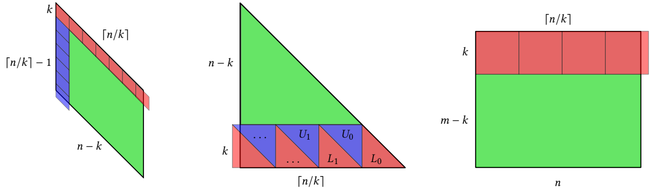
Figure 1: Tilings of the matrices \mathbb{M}_{FP}(f) (left), \mathbb{M}_{SP_{10}}(f) (center) and \mathbb{M}_{MP}(f) (right).
