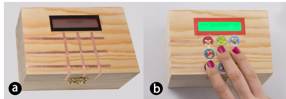
Figure 14. Wooden treasure box: (a) Rapid prototyping with copper tape on a wooden box, (b) touching three different images unlocks the box.
