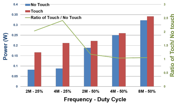
Figure 3. Total energy of receive signals in different frequencies and duty cycles. The greatest difference between the energy of touch and no touch signals belongs to the 4 MHz frequency with 25% duty cycle, which makes it a suitable choice for touch detection.
