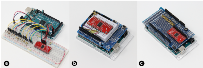
Figure 7. The simple hardware setup can be implemented on (a) a breadboard, (b) using an Arduino Proto Shield without soldering, and (c) with soldered connections.
