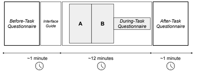
Figure 2: Task workflow.
