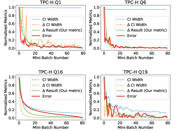
Figure 6: Several TPC-H queries' normalized absolute errors compared to ReLAQS's progress metric. A metric is a better estimate of progress if it more closely follows the red line labeled error.
