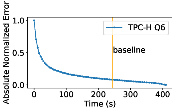
Figure 1: Normalized absolute error of an approximate query processing system running TPC-H query 6. The baseline here shows how long the same query takes in a traditional SQL-on-hadoop system.
