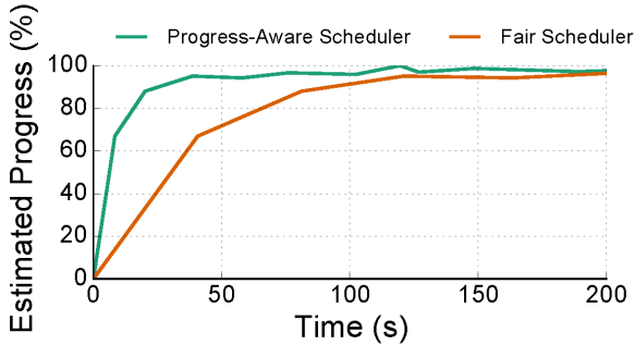
Figure 2: Giving more resources to queries with more error helps them get higher quality (i.e., less erroneous) results faster.
