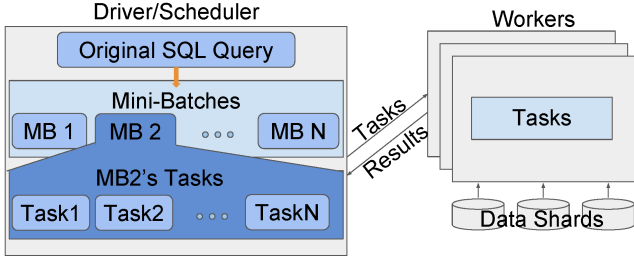
(a) When an approximate SQL query is submitted to the driver, its data is shuffled and partitioned into mini-batches on the driver. Each mini-batch is further partitioned into tasks, which are sent to the workers.
