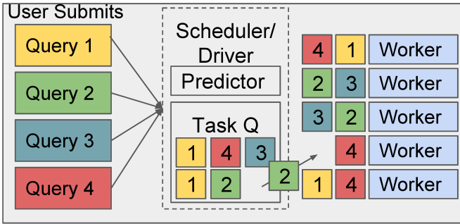
(b) ReLAQS's task queue sorts tasks by potential progress and assigns them to the workers.
