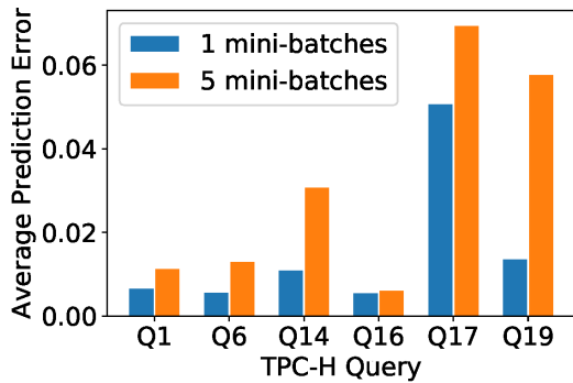
Figure 10: Several TPC-H queries' prediction errors. Average prediction for even noisy queries caps at 5% for 1 mini-batch in advance and 7% for 5 mini-batches in advance.
