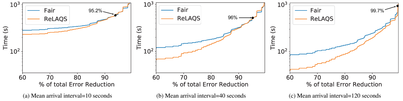
Figure 8: The average amount of time it takes to reach a particular error reduction with ReLAQS. Because scheduling is a zero-sum game, applications do take longer to reach error reduction above the crossing points of 95.2%, 96%, and 99.7% respectively, but significantly less time for other approximate results.
