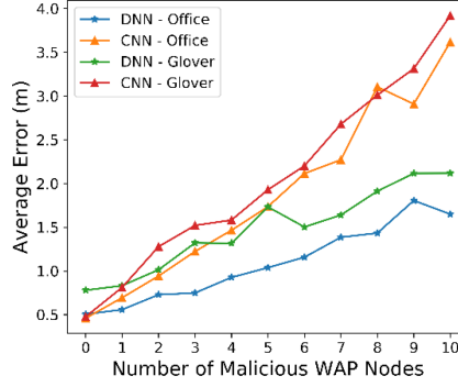
Fig. 7. Results for the impact of malicious WAPs on deep learning model accuracy on the Office and Glover paths. Average localization error for the CNN [15] and DNN [17] localization frameworks is shown for an increasing number of malicious WAPs.
