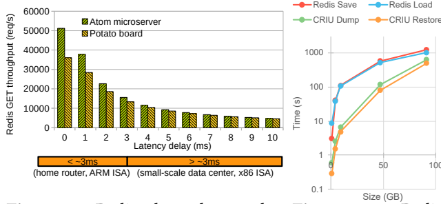
Figure 1. Redis throughput when varying client-server network latency. Figure 2. Redis persistence vs CRIU.
