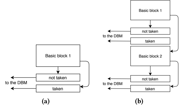
Figure 1. Basic blocks — (a) a newly created basic block; (b) the taken path directly linked to Basic Block 2.
