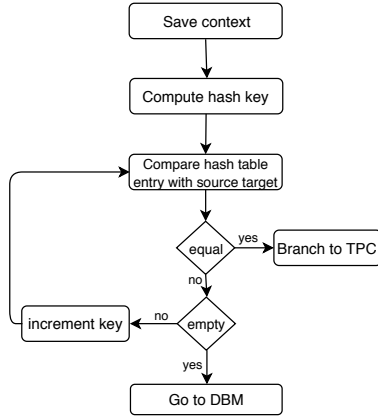
Figure 2. Inline hash lookup routine.
