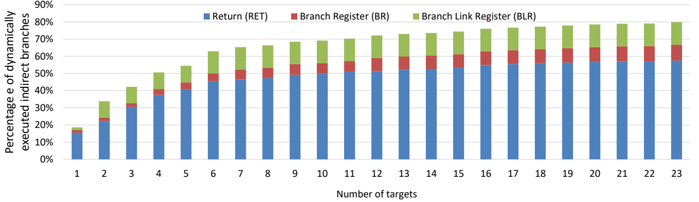
Figure 4. Percentage of dynamic indirect branches captured by inlining target predictions across SPEC CPU 2006.
