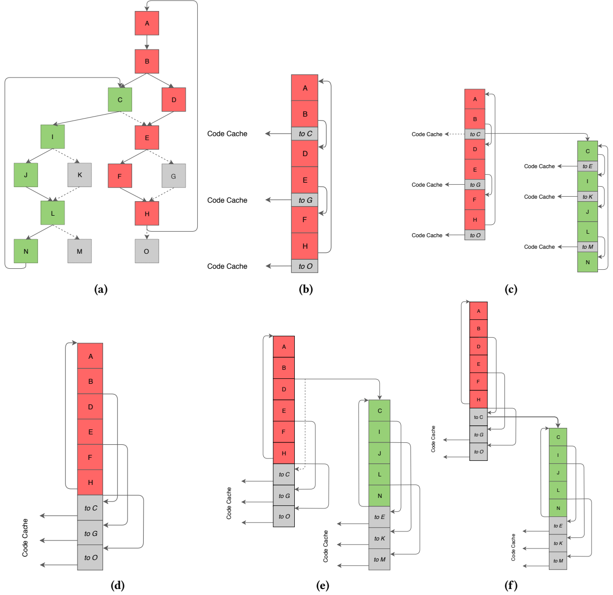
Figure 3. (a) Example control of flow from an application. Basic block are represented by boxes. (b) Trace layout of the first hot loop with the baseline scheme (interleaved). (c) Trace linking: once the second hot is identify and a trace is built, an exit from the first trace is linked to the trace entry of the second loop. The replaced path of the branch after linking is shown with a dotted line. (d) Contiguous Trace layout of the first hot loop. (e) Contiguous Trace linking scheme. The replaced path of the branch after linking is shown with a dotted line. (f) Linking a trace when the target is outside the range of a conditional direct branch.
