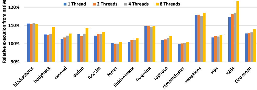
Figure 9. Scalability results — Relative execution time for PARSEC 3.0 on Applied Micro X-Gene 2 system with Contiguous Traces and the TRIBI 6 optimisation enabled for MAMBO.
