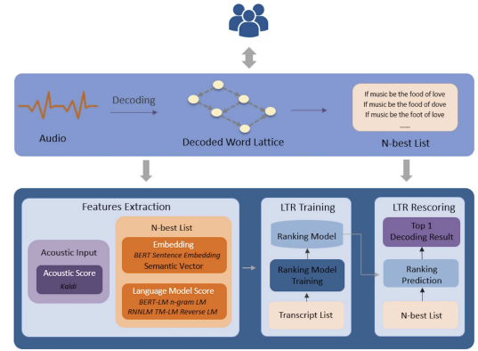
Figure 1: A System Overview of GoldenRetriever
