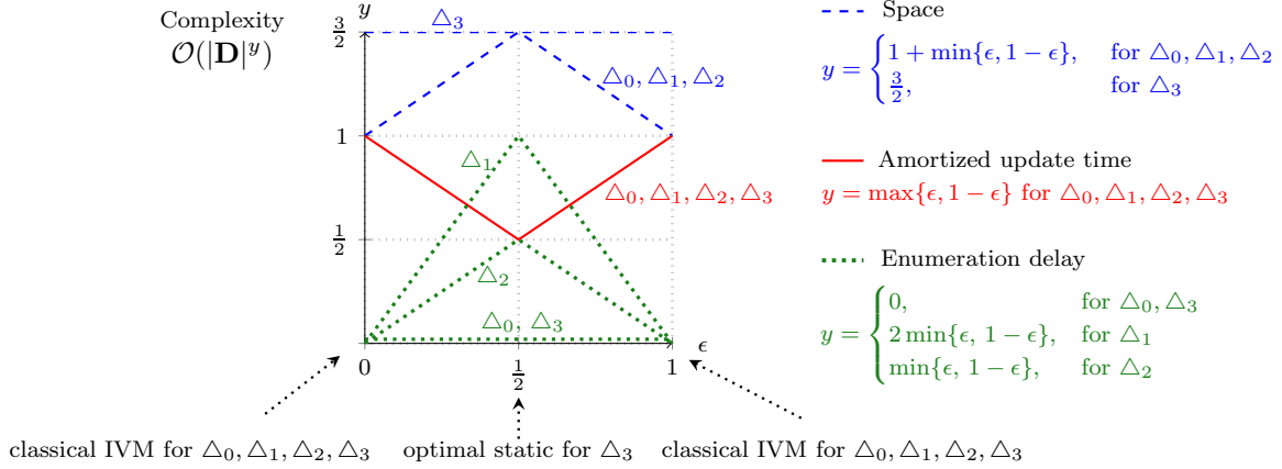
Figure 1: IVM^\epsilon 's amortized update time, space, and enumeration delay for maintaining triangle queries. |\mathbf{D}| is the database size. The complexities are parameterized by \epsilon . The space and enumeration delay depend on the arity of the query result. By setting \epsilon to 0 or 1, IVM^\epsilon recovers classical first-order IVM. For \epsilon = \frac{1}{2} , IVM^\epsilon computes the ternary triangle query worst-case optimally.
