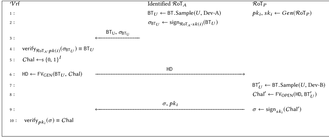
Figure 4: Proxy RTI protocol: \mathcal{Vrf} is assisted by a previously identified \mathcal{RoT}_A (residing on Dev-A) to decide whether \mathcal{RoTp} resides on physical device Dev-B. Dev-A, Dev-B, and user U must be physically co-located. \mathcal{Vrf} can be remote.
