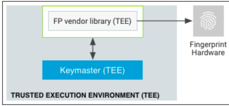
Figure 2: TEE-Biometric hardware architecture of a typical Android device (adapted from [18])
