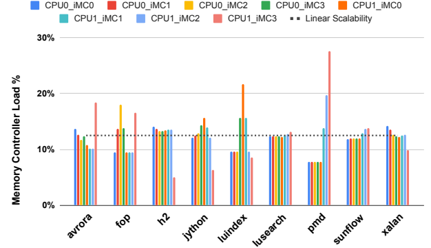
Figure 8: Dacapo memory controller load in dual node.
