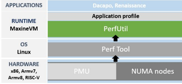
Figure 3: The proposed profiling infrastructure.
