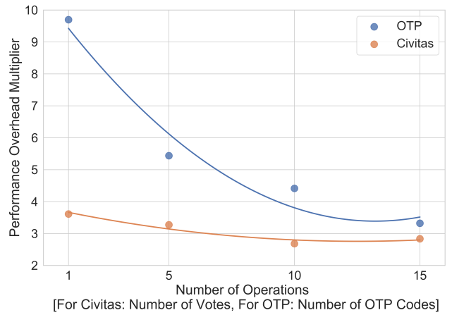
Figure 6: Performance Overhead Graph
