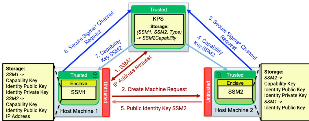
Figure 4: Trusted Create Protocol
