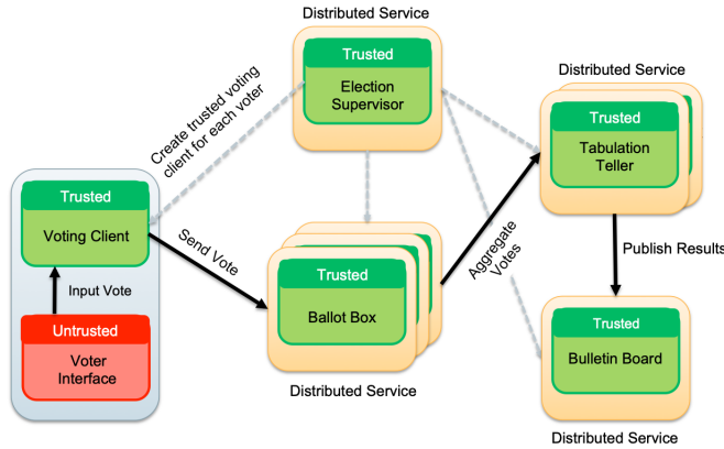
Figure 1: Civitas Architecture
