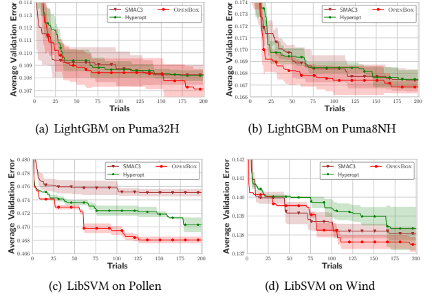
Figure 12: Performance of two AutoML tasks on 4 datasets. obtains a 3.8 \times speedup over SMAC3 when achieving the comparable convergence performance.
