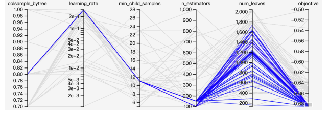
Figure 4: An example of the Parallel Coordinates Visualization for configurations when tuning LightGBM .
