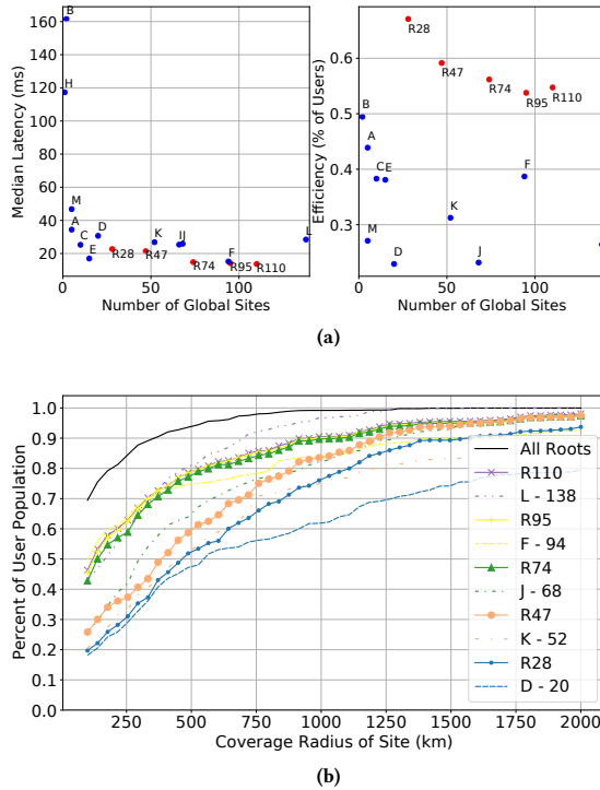
Figure 7: Larger deployments lead to lower latency (Fig. 7a-left) since they offer more low-latency options to users (Fig. 7b). However, fewer users visit their closest site (Fig. 7a-right) leading to more inflation.
