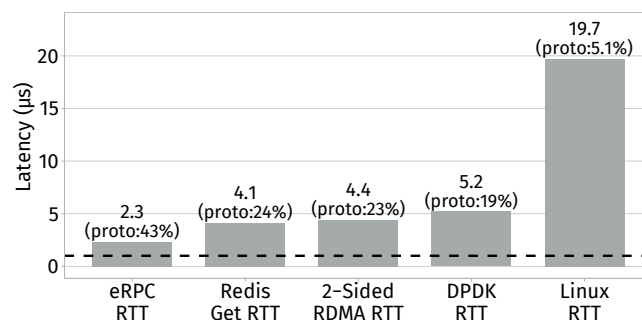
Figure 1: Reported RTTs of recent microsecond-scale systems, annotated with the percentage overhead that Protobuf serialization and deserialization of a single 1024 byte string (1.0 μs) would add (shown in the dashed line). Redis RTT comes from Arrakis [27], eRPC from eRPC [17], while the RDMA, DDPK and Linux RTTs are measured on the Demikernel. [42].
