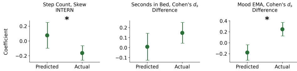
Fig. 7. Plots of the shared significant coefficients from GEE using calculated features from the actual and predicted data. All features were either calculated using generated data from the internship (INTERN) or a difference between the internship and baseline periods (Difference). (a) shows the coefficient differences from the univariate and (b) from the multivariate GEE. There is a single plot per feature. The y-axis on each plot is the resulting \beta coefficient from conducting GEE to measure the effect of the feature from distinguishing stress-resilient versus sensitive individuals. The x-axis dictates whether the plotted values are from the GEE using the actual or predicted values. Points are the mean value of the coefficient, and error bars represent 95% confidence intervals. * indicates that the coefficients are significantly ( \alpha = 0.05 ) different.
