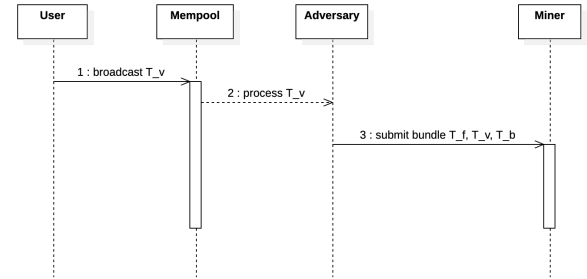
Figure 8: A sequence diagram illustrating how adversaries guarantee transaction order by participating in sealed-bid auctions to compete for block space.
