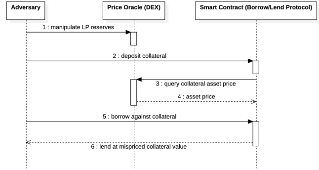
Figure 10: A sequence diagram depicting an example of an oracle manipulation exploit; involving an adversary, and a lending/borrowing smart contract to be arbitrated which queries an on-chain price oracle.
