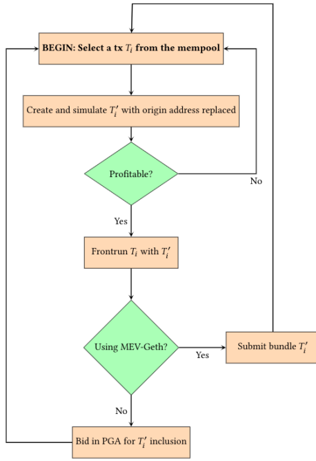
Figure 5: Flowchart of the cosmic horror lurking in the Dark Forest; the generalised frontrunner.
