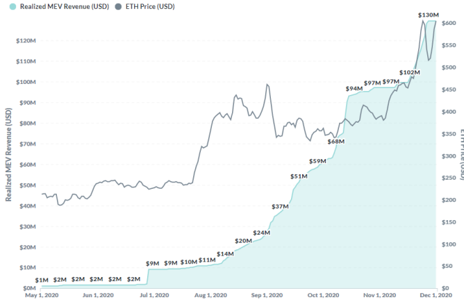
Figure 3: The exponential growth of MEV revenue in 2020 (from Paradigm Research [21])
