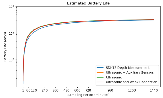
Figure 8: Battery Life estimates for varied sampling rates
