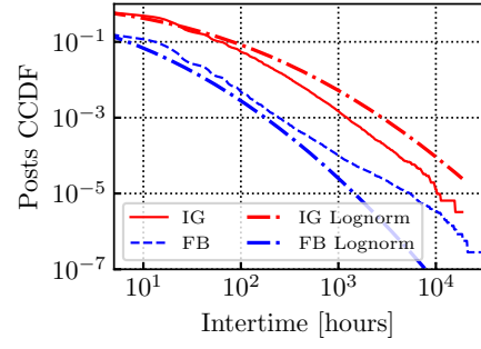
Fig. 3: CCDF of the posts intertime for the influencers (loglog scale).
