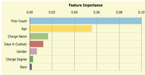
(b) Explanation: Feature importance
