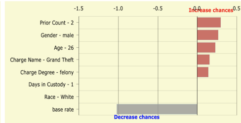
(c) Explanation: Feature contribution
