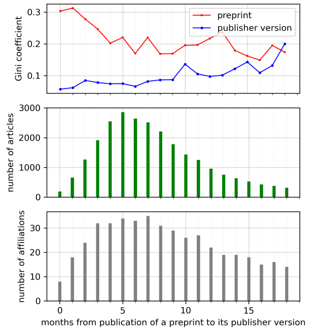
Figure 4: Gini coefficients of citations of preprints and publisher versions grouped by months from publication of a preprint to its publisher version at country level.
