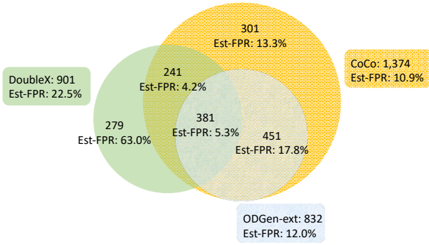
Figure 4: Venn diagram of reported results (including false positives) of CoCo, ODGen-ext, and DoubleX on the large-scale extension dataset. We annotate the estimated False Positive Rate (Est-FPR)—which is obtained manually by randomly sampling 10% reports—under each number.
