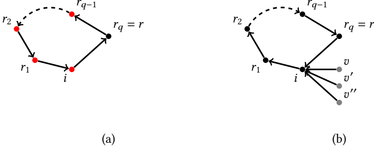
Fig. 3. The figures show (part of) the orientation graphs of the allocations X (a) and X' (b) for the first scenario of the orientation graph of X in Lemma 11. The red vertices represent agents that are envied by some other agent, the black vertices are not envied by anyone and the gray vertices may be either envied or non-envied (may be either red or black).
