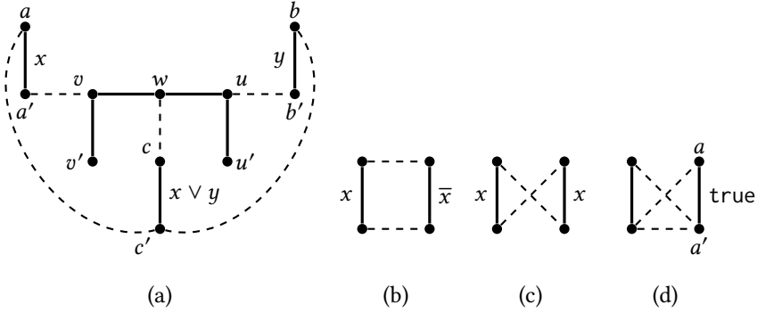
Fig. 2. In these figures, heavy edges (with some fixed high value v \gg 1 for both agents) are represented by thick lines and light edges (with value 1 for both agents) are represented by dashed lines. true corresponds to orienting an edge towards its upper node. (a) OR gadget: edge x \vee y is given to agent c if and only if edge x is given to agent a or edge y is given to agent b . Furthermore, there is an EFX allocation for every orientation of edges x and y . (b) NOT gadget. (c) consistency gadget. (d) true gadget: in every EFX orientation the edge (a, a') must be oriented towards a .
