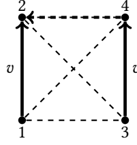
Fig. 1. The weight of heavy edges is v \gg 1 for both agents and they are represented by thick lines. The light edges carry low weight (with value 1 for both agents) and they are represented by dashed lines. No matter how the two thick edges are oriented, this will create envy. In the figure, agents 2 and 4 receive the thick edges. Note that one of them needs to also receive the light edge (2, 4). In the figure, it is given to agent 2. Now observe that irrespectively of the orientation of the rest of the edges, agent 1 envies agent 2 (even if edge (2,4) is removed), so EFX is violated.
