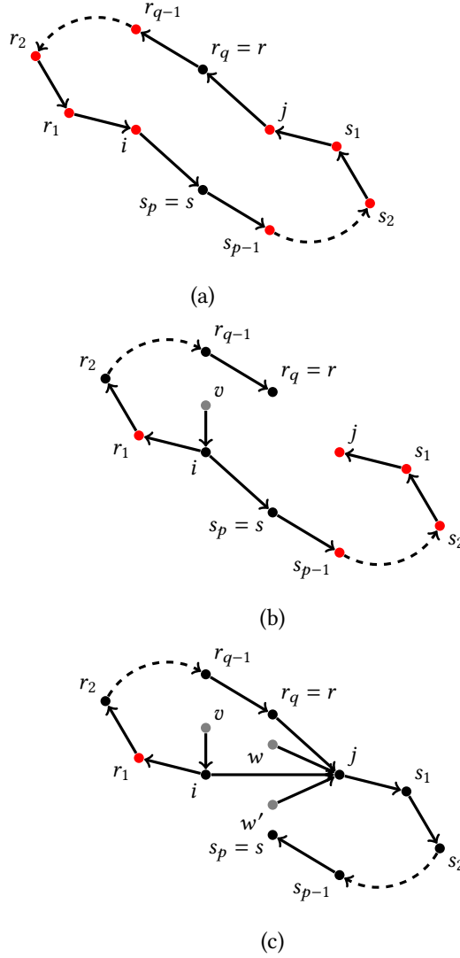
Fig. 4. The figures show (part of) the orientation graphs of the allocations X (a) and X' (where (b) and (c) refer to X' when i doesn't prefer or prefers, respectively, (i, s) to (i, j) ) for the second scenario of the orientation graph of X in Lemma 11. The red vertices represent agents that are envied by some other agent, the black vertices are not envied by anyone and the gray vertices may be either envied or non-envied (may be either red or black).
