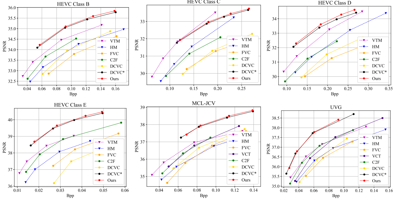
Figure 4: Rate-distortion (i.e., bitrate vs PSNR) performance comparison of our and other state-of-the-art methods in the HEVC, MLC-JCV, and UVG datasets.
