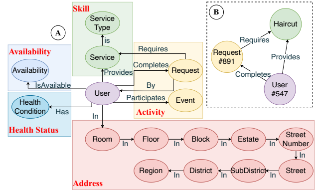
Figure 2: HIN Schema and Example
