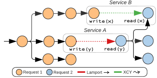
Figure 3. This example illustrates the difference between Lamport's \rightarrow and XCY's \leadsto . While the red dependency is present in both definitions, the green dependency stems from the concept of lineage and is only present in \leadsto .
