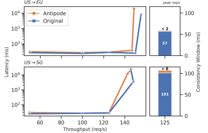
Figure 8. (Left) Average throughput vs. Latency and (Right) Consistency window (at peak 125 req/s) in the original DeathStarBench, and with Antipode enabled. Results split between US→EU and US→SG replication pairs.
