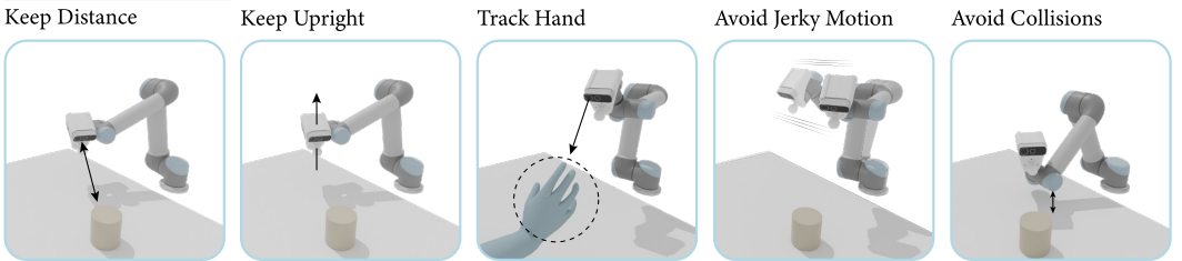
Fig. 3. The Periscope system supports a variety of interactions for the helper and the worker, assisted by autonomous robot behaviors. Images with a blue border represent the local workspace, where both the robot and the worker are present. Images in the top row with a green border depict the remote helper's UI which enables the helper to interact with the system through mouse input on the camera feed or the control panel. Worker interactions leverage the worker's proximity to the robot, allowing them to move the camera directly using gestures and physical contact with the robot arm. Autonomous behaviors focus on geometric (rather than semantic) qualities of the view, which are challenging for humans but feasible for robots to achieve.
