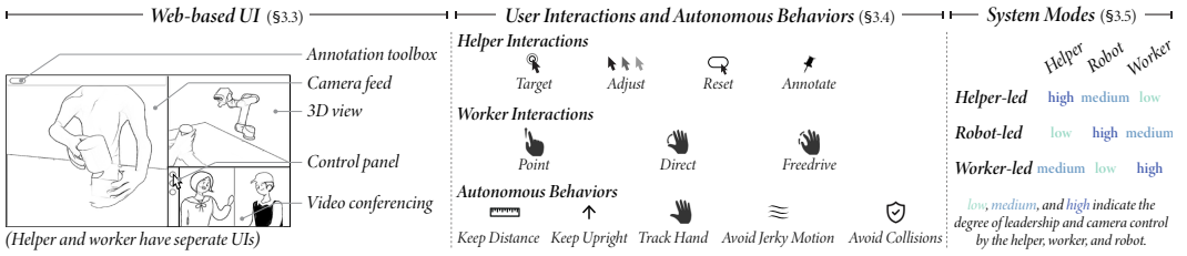
Fig. 2. The Periscope system consists of three components: user interfaces for the helper and the worker, a set of helper interactions, worker interactions, and autonomous robot behaviors to support establishing a shared visual context, and system modes that arbitrate user interactions and autonomous behaviors in real-time, resulting in camera motion. (Left) Each user interface includes a camera feed that displays the live video feed from the robot-mounted camera, accepts mouse input commands, and can be annotated using the annotation toolbox ; a 3D view that shows a visualization of the robot and its surroundings; a video conferencing panel for verbal communication between the helper and the worker; and a control panel for mode selection. (Center) Helpers use the screen interface to interact with the system via mouse input commands on the camera feed or the control panel. Workers move the camera by engaging directly with the robot arm using physical contact and gestures. Autonomous robot behaviors augment helper and worker interactions by supporting the aspects of camera control that are difficult and non-intuitive for users. (Right) Helper-led Mode , Robot-led Mode , and Worker-led Mode are three system modes that arbitrate user interactions and autonomous behaviors differently, offering varying degrees of control to both users for low effort. Users can select from the three available modes via the control panel to support their current needs.
