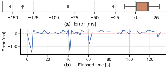
Figure 4: Timing accuracy (i.e., error) of librnr as a statistical summary (top plot) and over time (bottom plot).
