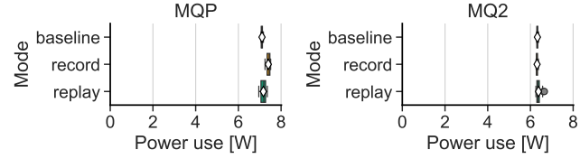
Figure 5: librnr energy overhead on Meta Quest Pro (MQP) and Meta Quest 2 (MQ2).
