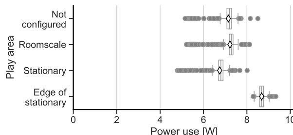
Figure 1: Meta Quest Pro power use when using different play area configurations.
