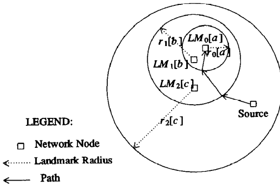
Figure 3: Landmark Hierarchy
