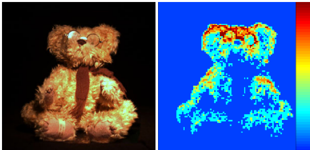
Figure 9: a) Original view. b) Visualization of number of PCA components per block (Max. = 15, Mean = 5).
