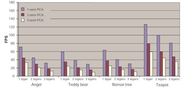
Figure 9: Rendering performance of opacity light field mapping using Nvidia GeForce4 Ti 4600 graphics card on a 2GHz Pentium 4 PC displayed at 1024 \times 768 window with objects occupying approximately 1/3 of the window.
