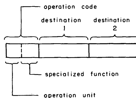
Figure 4. Instruction format.
