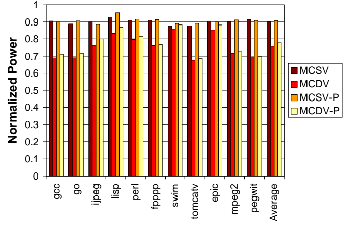
Figure 5. Normalized power
