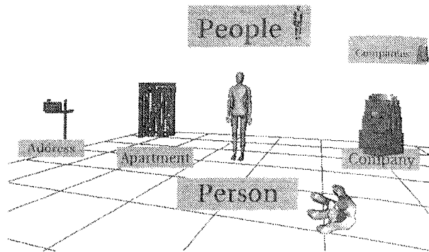
Figure 17: Database Schema
