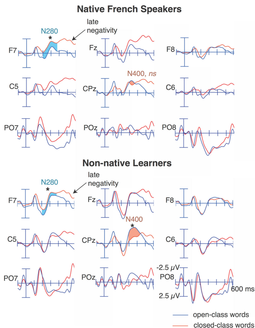
Figure 2. ERPs time-locked to open- and closed-class words. ERPs demonstrate word class effects (the N280, the N400, and the late negative shift) in both native speakers and in L2 learners, providing a general picture of processing.
