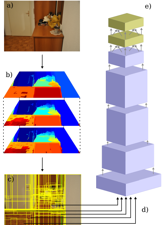
Figure 6. Vision-based part extraction pipeline. (a) Input RGB image. (b) Selective search (Uijlings et al., 2013) performs hierarchical grouping of segmented images at different scales. (c) Proposed image regions. (d) Regions are fed into a CNN (Zhou et al., 2014) that performs feature extraction. (e) The vision-based part is represented with the output of the last fully connected network layer for the corresponding input region.
