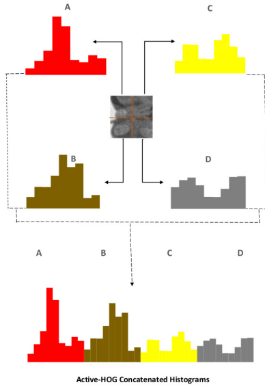
Figure 9. Active-HOG histograms of the active window image patch and the concatenated histograms.
