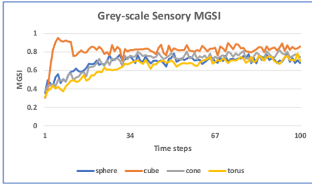
(a) Modified Geometric Separability (MGSI) of the stimuli provided by the greyscale averaging method
