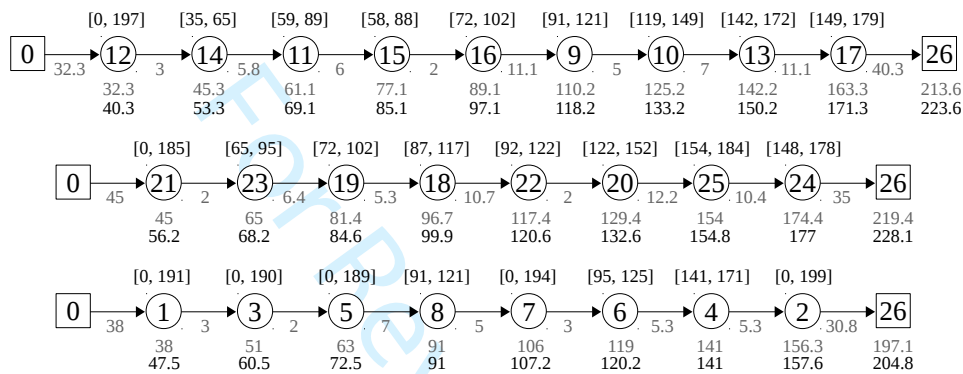
Figure 6 Optimal solution of instance RC102 for \Gamma^t = 1 with an optimal value of 352.0 (PoR of 0.06%) and a risk of 50.47%.
