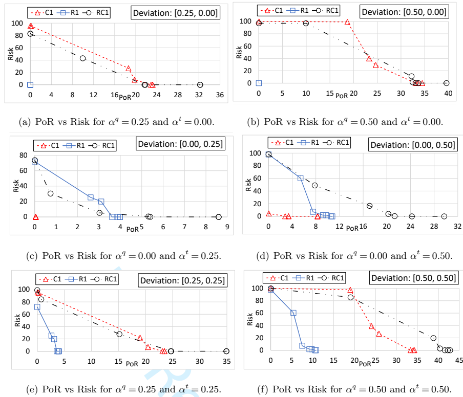
Figure 3 Trade-off between price of robustness (PoR) and probability of constraint violation (Risk) for 100-series set instances with 25 customers.
