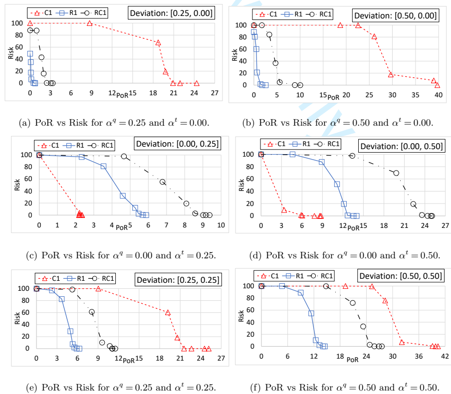
Figure 4 Trade-off between price of robustness (PoR) and probability of constraint violation (Risk) for 100-series set instances with 100 customers.
