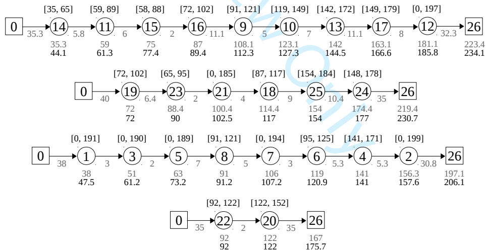
Figure 7 Optimal solution of instance RC102 for \Gamma^t = 2 with an optimal value of 401.8 (PoR of 14.21%) and a risk of 0.01%.
