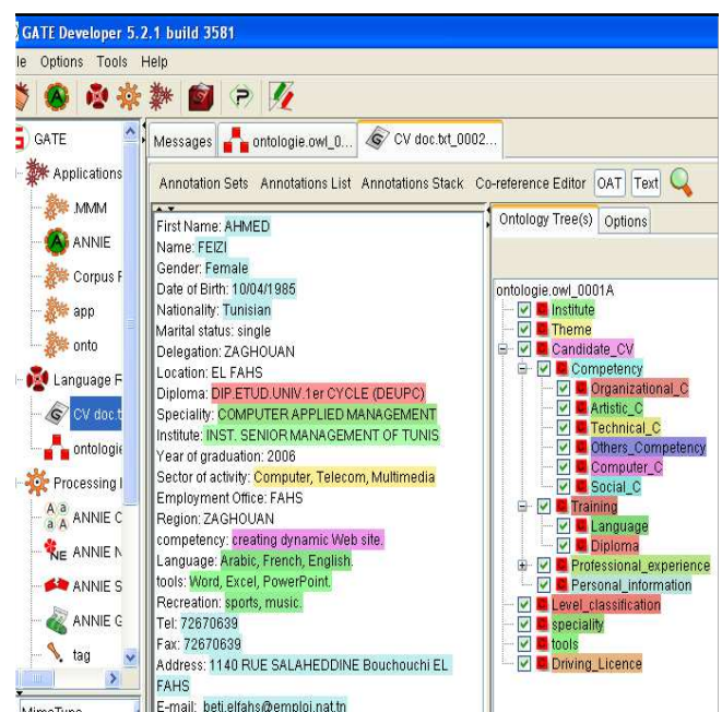
Fig. 6. Annotating using Gate API (OAT)
