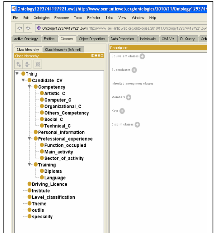
Fig.2.: ERECO Ontology with aptitude and Competencies
