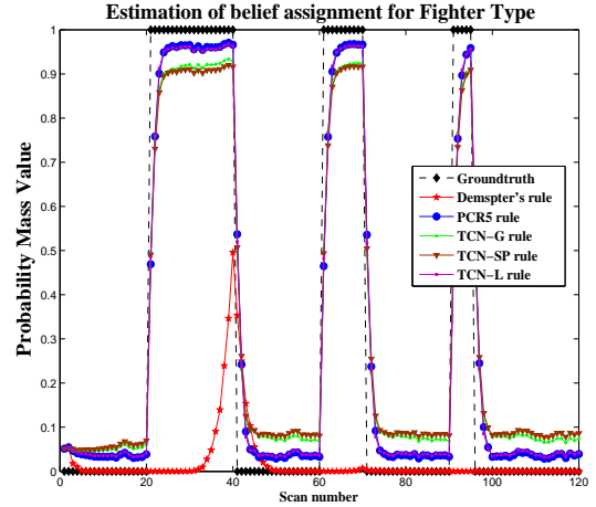
Figure 2: Estimation of belief assignment for Fighter type.
