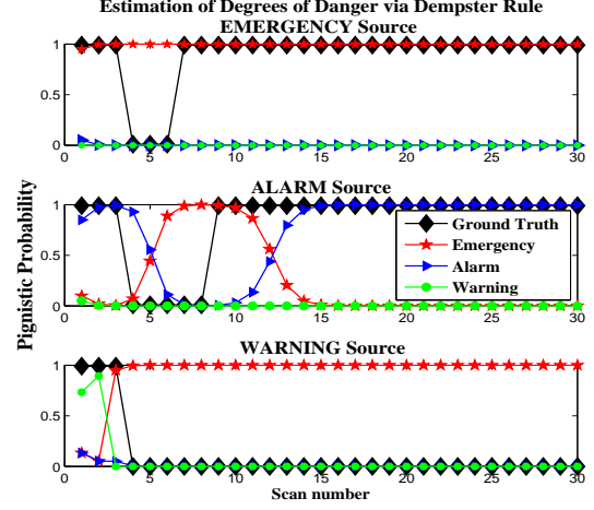
Figure 6: Dempster's rule Performance for danger level estimation.
