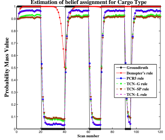
Figure 1: Estimation of belief assignment for Cargo type.
