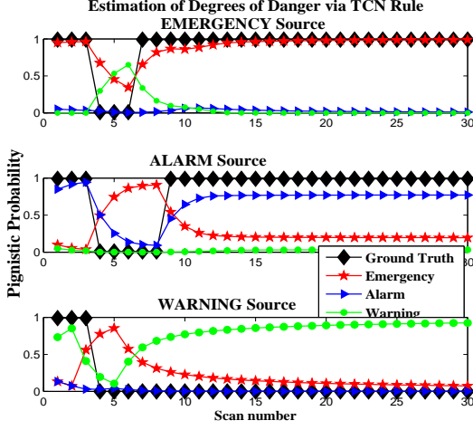
Figure 4: TCN rule Performance for danger level estimation.
